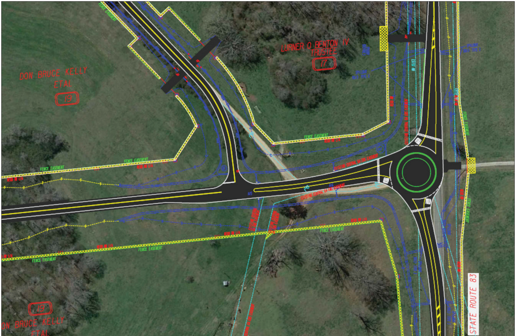
The new intersections at SR 380/SR 16 and SR 83 (pictured) will be roundabout designs, which could reduce current truck traffic through the city by up to 20%, according to GDOT engineers.
